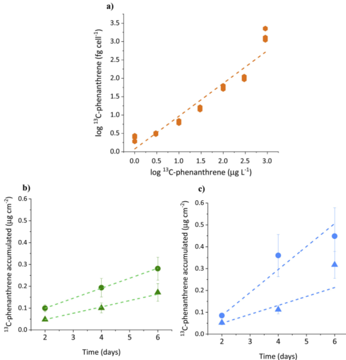
Fig. 2. Accumulation of ^{13}\text{C} -phenanthrene in microalgae and corals. (a) Fitted linear regression showing the relationship between a accumulation of ^{13}\text{C} -phenanthrene in D. salina cells ( \text{fg cell}^{-1} ) and ^{13}\text{C} -phenanthrene concentration in seawater ( \mu\text{g L}^{-1} ). Uptake of ^{13}\text{C} -phenanthrene by A. millepora fragments, as mean \pm SE accumulated ^{13}\text{C} -phenanthrene ( \mu\text{g cm}^{-2} ) over time (days), through (b) dietary exposure (via labelled D. salina ) and (c) aqueous exposure, at the nominal phenanthrene concentrations of 18.2 \mu\text{g L}^{-1} (triangles \blacktriangle , \blacktriangle ) and 44 \mu\text{g L}^{-1} (circles \bullet , \bullet ). Lines represent the linear fitted regression.
