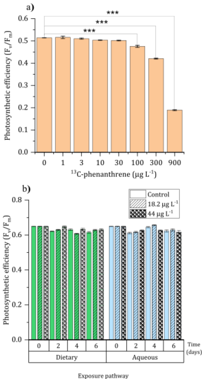
Fig. 1. Changes in photosynthetic efficiency ( F_v/F_m ) (mean \pm SE) of D. salina cultures and coral fragments observed in controls and when exposed to ^{13}\text{C} -phenanthrene. (a) Bar graph showing decline in F_v/F_m in D. salina cultures exposed to a range of ^{13}\text{C} -phenanthrene concentrations. (b) Grouped bar plot of F_v/F_m in A. millepora fragments exposed to ^{13}\text{C} -phenanthrene via dietary (green bars) and aqueous (blue bars) exposure pathways. Bars marked by *** show < 0.001 significant difference from all other treatment concentrations at 0.05 level analyzed by one-way ANOVA and Tukey's posthoc test for pair-wise differences. (For interpretation of the references to color in this figure legend, the reader is referred to the Web version of this article.)
